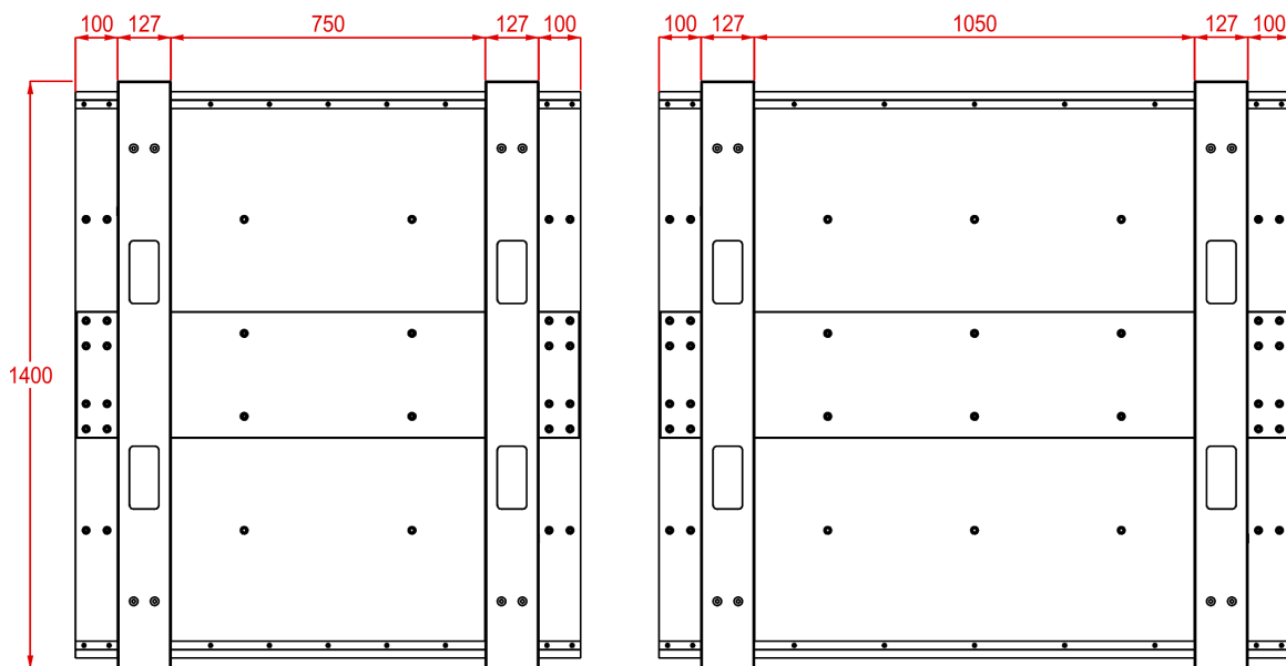
Cable entry points and sizes
