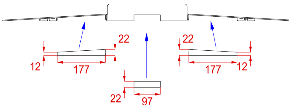
Cable entry points and sizes
